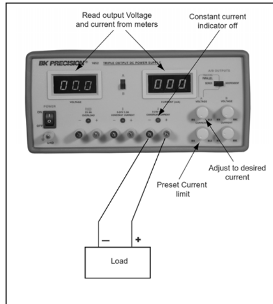
Figure 4. Typical constant voltage operation
