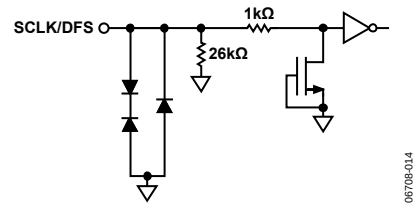
Figure 15. Equivalent SCLK/DFS Input Circuit
