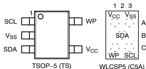
TSOP-5 (TS)
