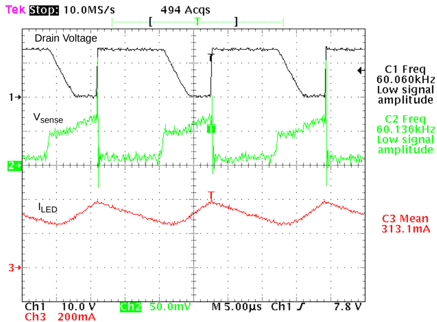
Figure 12. NUD4021, Typical Operation Waveforms ( V_{CC} = 13.5\text{ V} , V_{LED} = 3.5\text{ V} , R_{sense} = 1.2\text{ }\Omega , R_{pullup} = 1.1\text{ k}\Omega , C_{in} = 100\text{ }\mu\text{F} , L = 330\text{ }\mu\text{H} )
