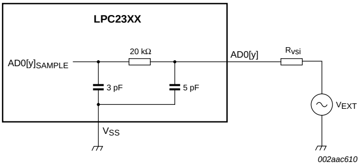
Fig 18. Suggested ADC interface - LPC2388 AD0[y] pin
