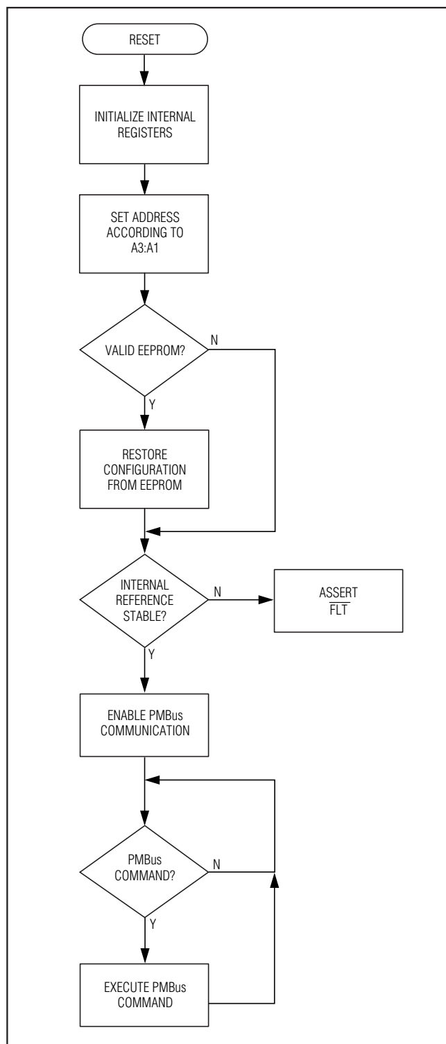
Figure 9. MAX8688 Initialization
