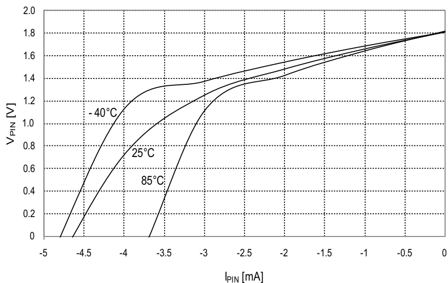
Figure 33-105. I/O pin output voltage vs. source current.
