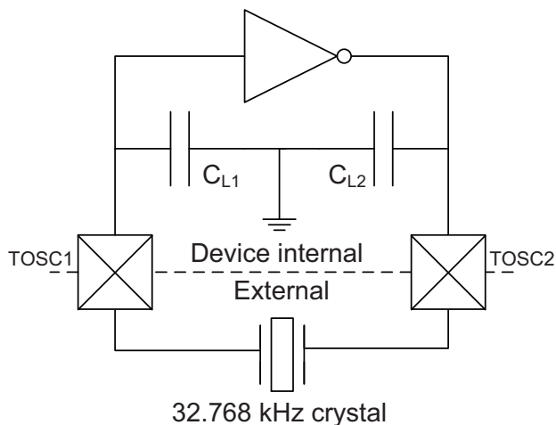
Figure 32-11.TOSC input capacitance.
