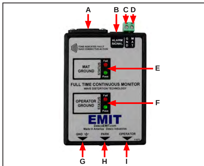
Figure 2. Full-Time Continuous Monitor features and components
