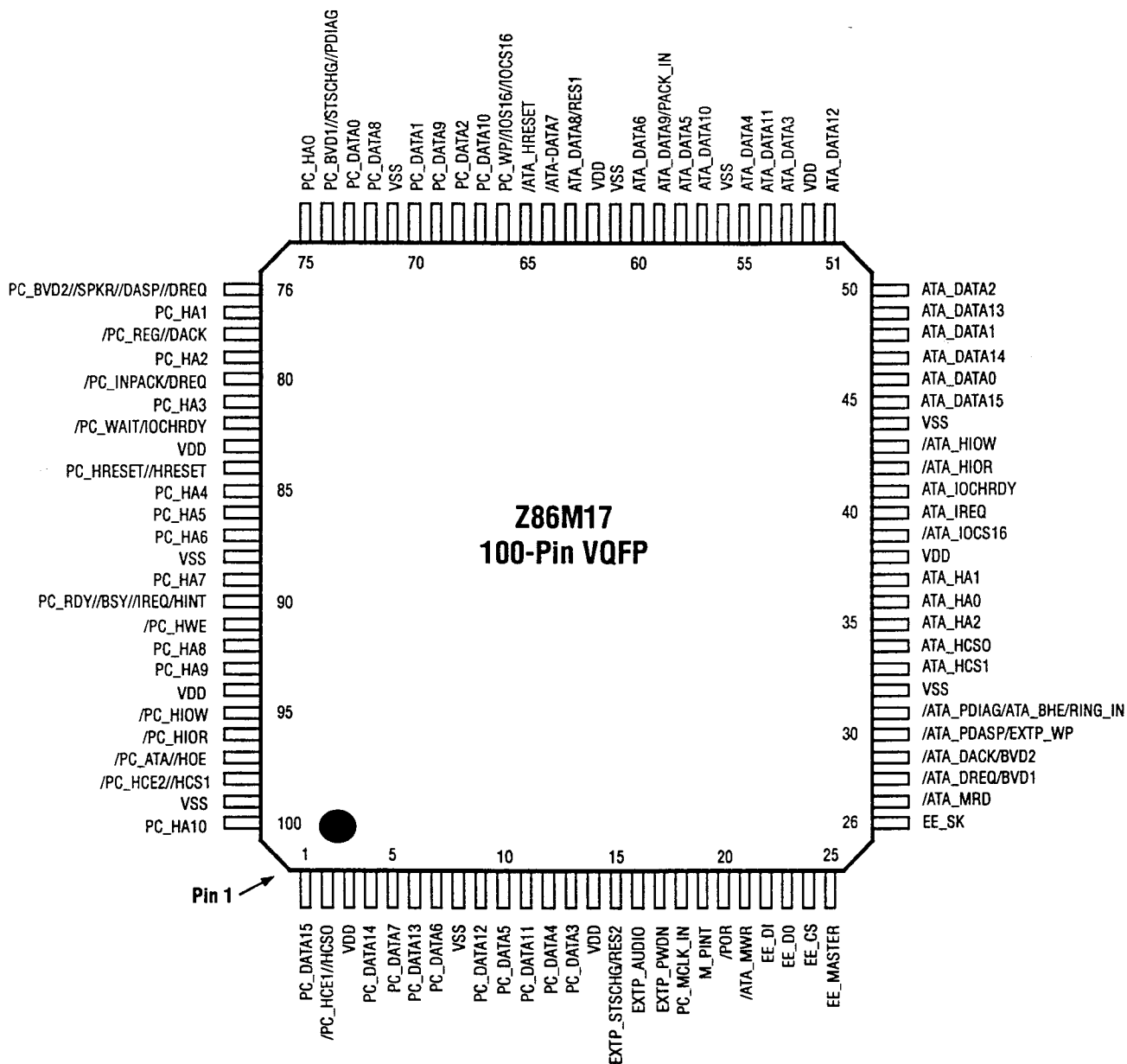
Z86M1720ASC 100-Pin VQFP Package
