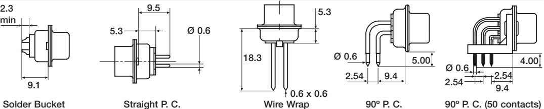
Solder Bucket
