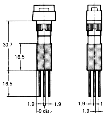
Wire-wrap Terminal
