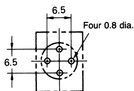
Mounting Hole (Bottom View)
