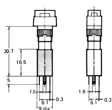
Solder Terminal
