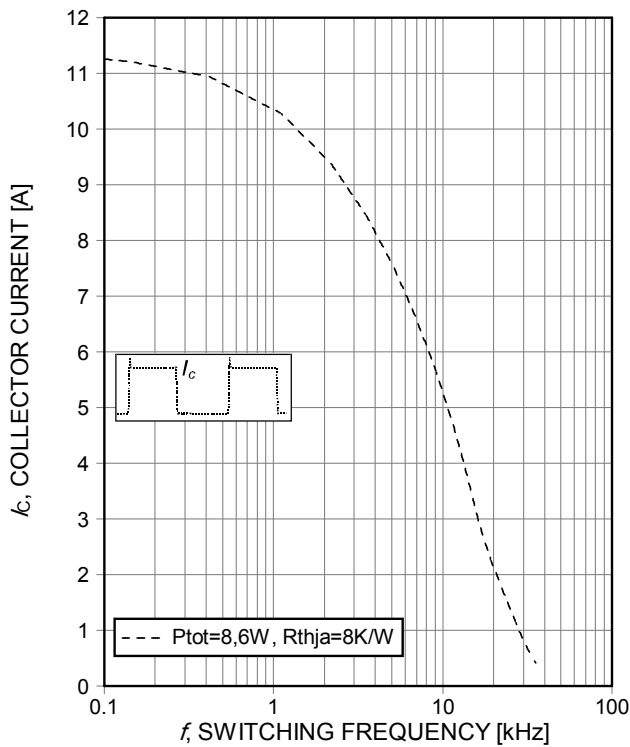
Figure 1. Collector current as a function of switching frequency (T_{vj} \leq 175^\circ C, T_a = 55^\circ C, D = 0.5, V_{CE} = 400V, V_{GE} = 15/0V, r_G = 15\Omega, \text{PCB mounting with thermal vias and heatsink, see Appnote: } \text{www.infineon.com/igbt})
