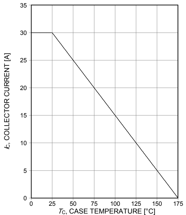
Figure 4. Collector current as a function of case temperature (V_{GE} \geq 15V, T_{vj} \leq 175^\circ C)
