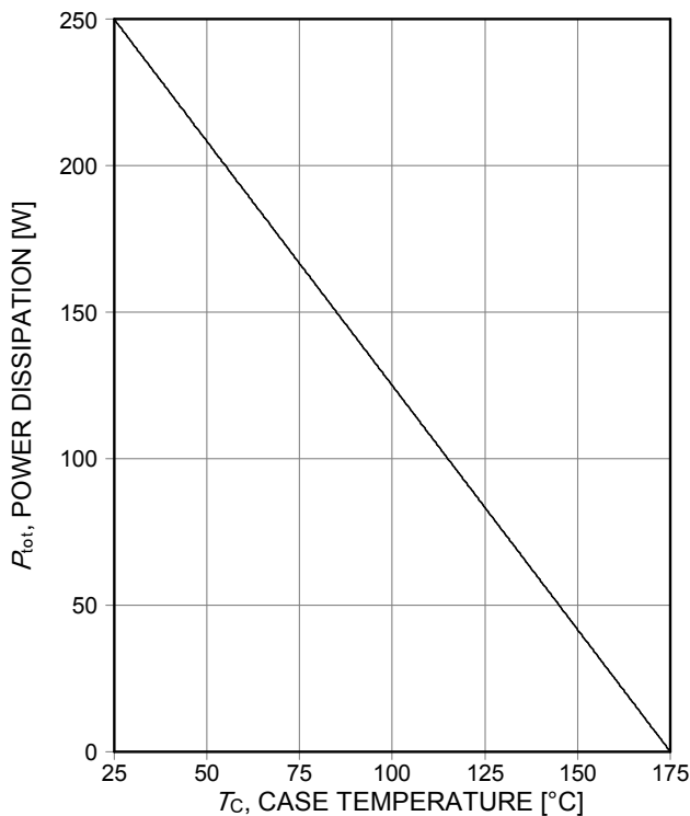
Figure 3. Power dissipation as a function of case temperature (T_{vj} \leq 175^\circ C)
