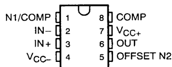
LM101A W FLAT PACKAGE (TOP VIEW)
