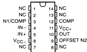
LM101A U FLAT PACKAGE (TOP VIEW)
