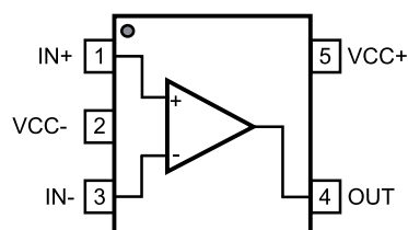
SC70-5
