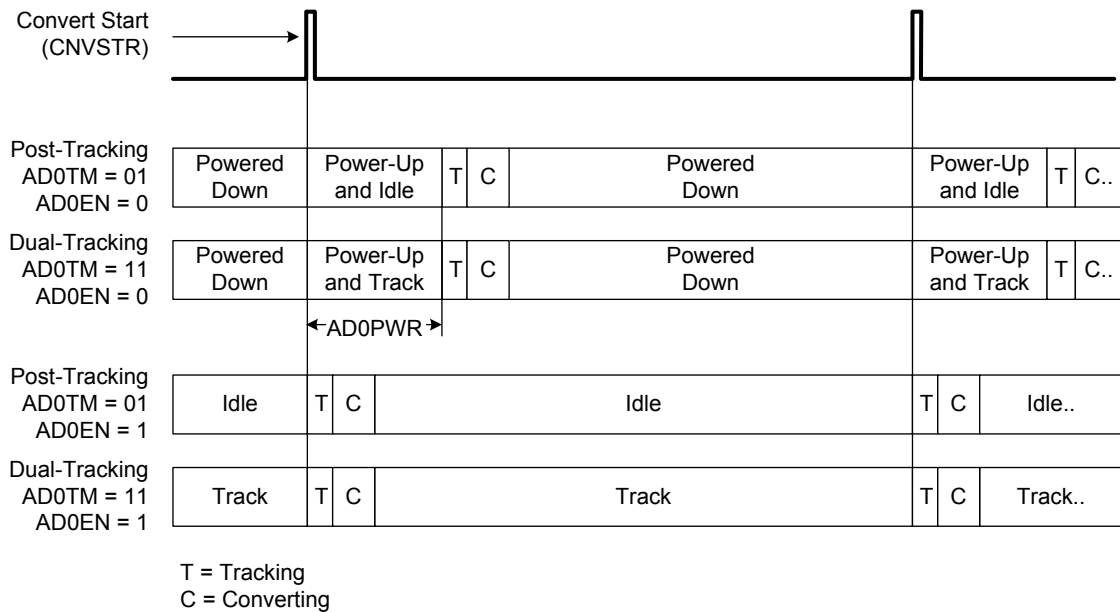
Figure 5.3. Burst Mode Tracking Example with Repeat Count Set to 4
