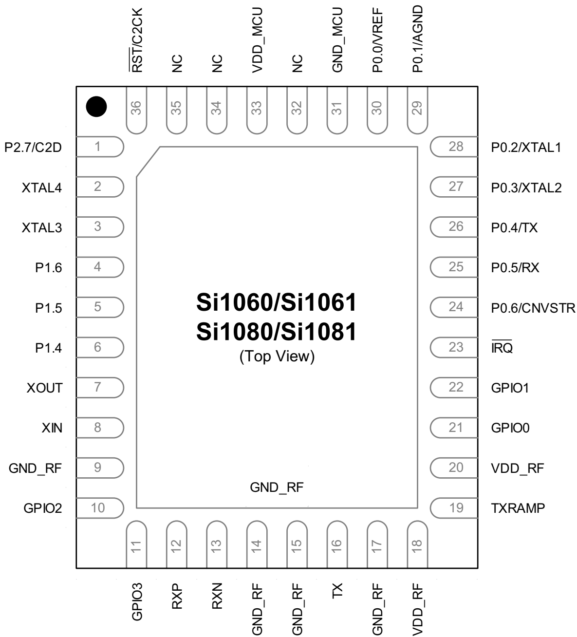
Figure 3.1. Si1060/1, Si1080/1-A-GM Pinout Diagram (Top View)
