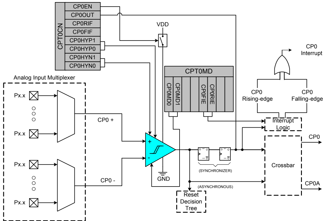
Figure 1.8. Comparator 0 Functional Block Diagram
