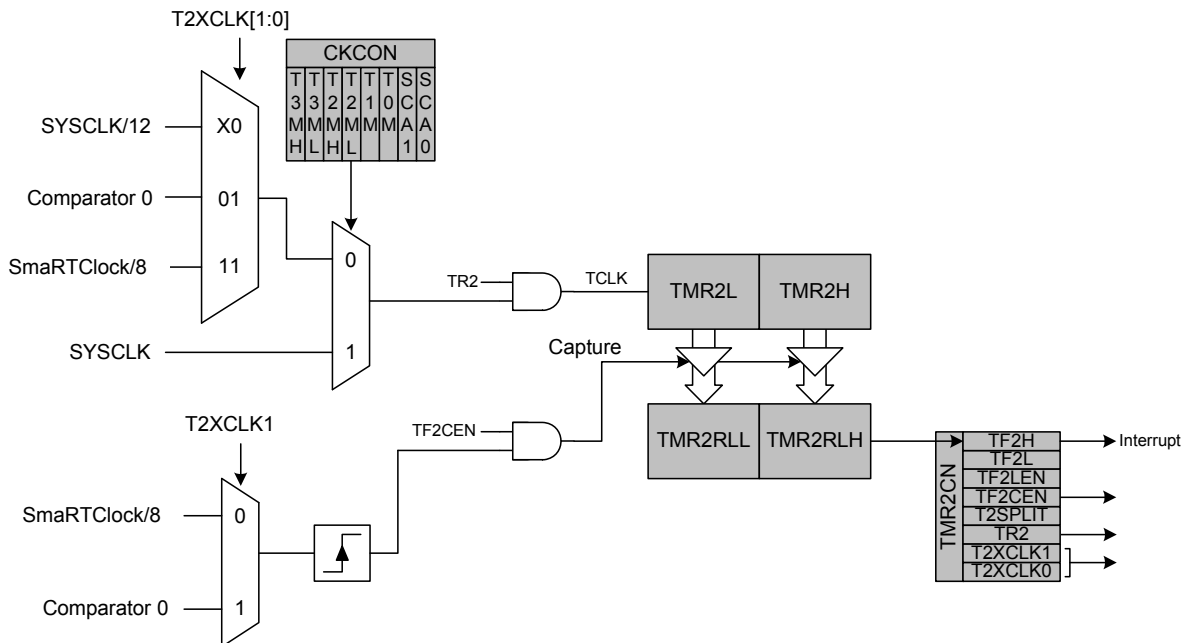
Figure 31.6. Timer 2 Capture Mode Block Diagram
