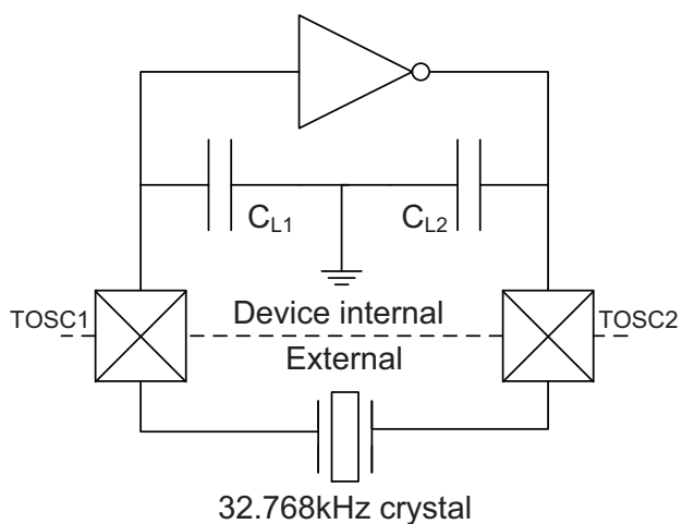
Figure 32-11.TOSC input capacitance.
