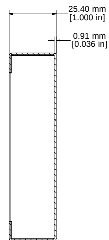
SECTION EE-EE
