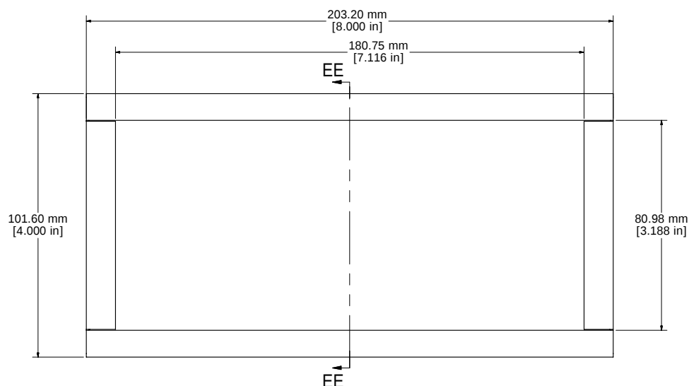
1441-9 OR 1441-9BK3 - VIEW FROM TOP (SOLD SEPERATELY)
