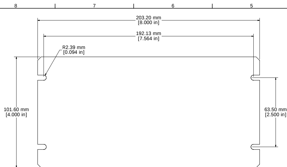
1431-10 OR 1431-10BK3 - VIEW FROM TOP (SOLD SEPERATELY)
