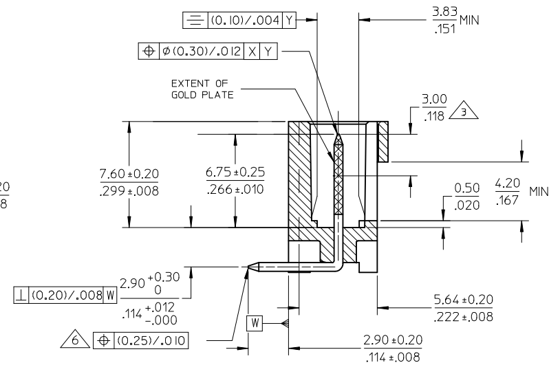
SECTION K-K
