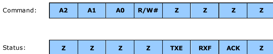
Figure 6.7 SPI Command and Status Structure
