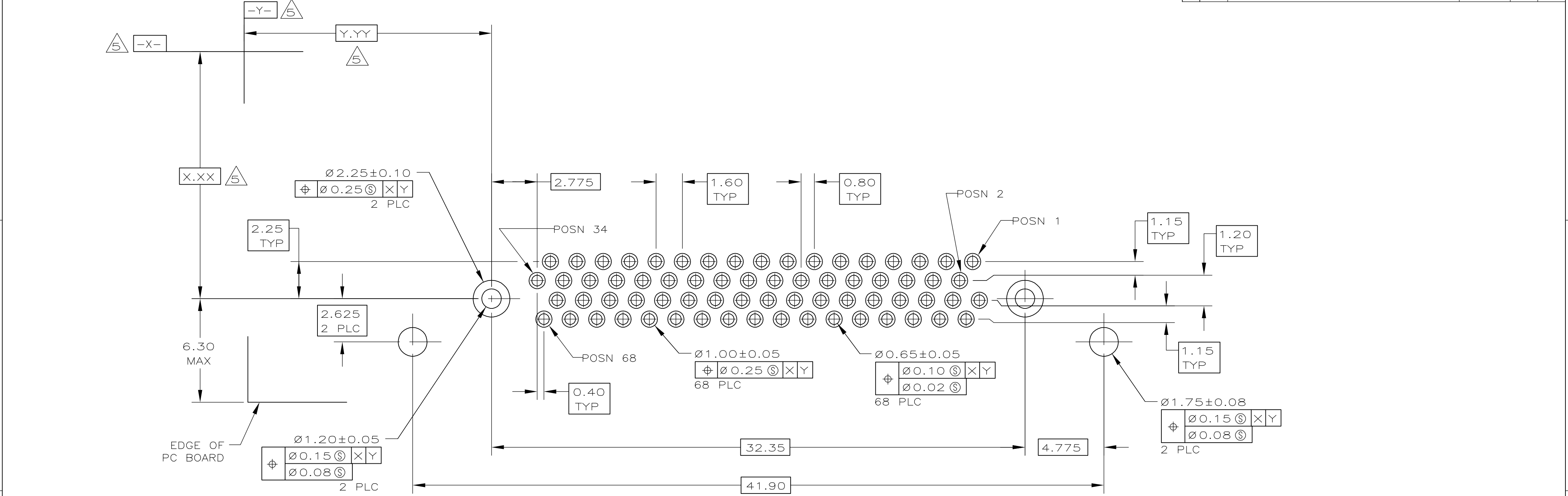
PC BOARD MOUNTING DIMENSIONS
