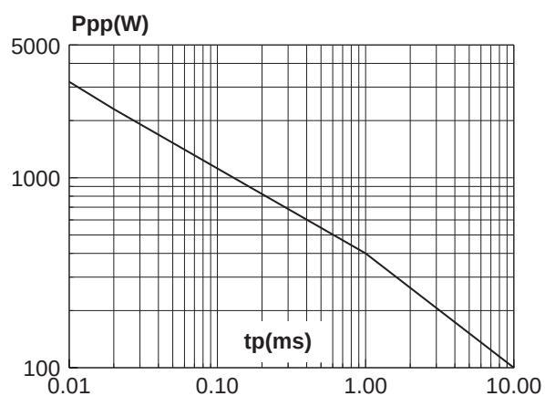
Fig 2: Peak pulse power versus exponential pulse duration ( T_j \text{ initial}=25^\circ\text{C} ).
