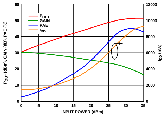
Figure 24. Power Compression at 2.7 GHz
