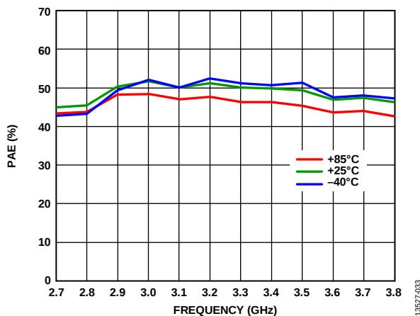
Figure 23. PAE vs. Frequency at Various Temperatures, PAE at P_{SAT} Defined as Output Power at P_{IN} = 31 dBm at 25°C, P_{IN} = 32 dBm at 85°C, and P_{IN} = 29 dBm at -40°C
