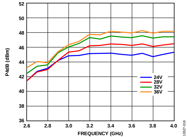
Figure 18. P4dB vs. Frequency at Various Supply Voltages
