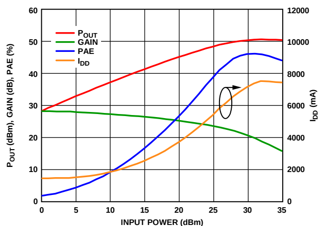
Figure 25. Power Compression at 3.8 GHz
