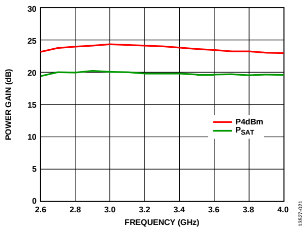
Figure 21. Power Gain vs. Frequency, Power Gain at P_{SAT} Defined as Output Power at P_{IN} = 31 dBm at 25°C
