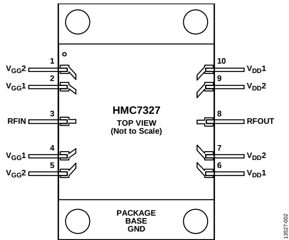
Figure 2. Pin Configuration
