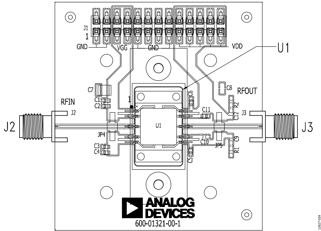
Figure 34. Evaluation PCB
