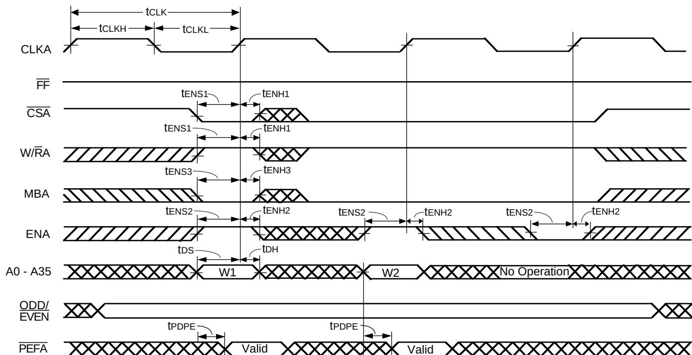
Figure 2. FIFO Write Cycle Timing
