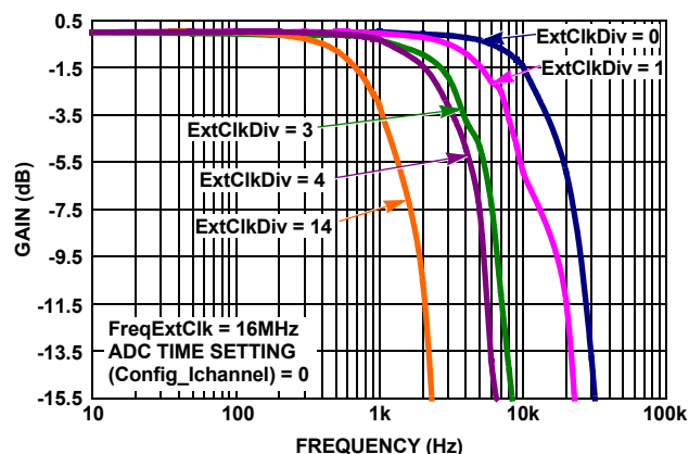
FIGURE 114. MEASUREMENT BANDWIDTH vs EXTERNAL CLK FREQUENCY
