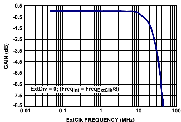
FIGURE 115. EXTERNAL CLOCK BANDWIDTH vs MEASUREMENT ACCURACY
