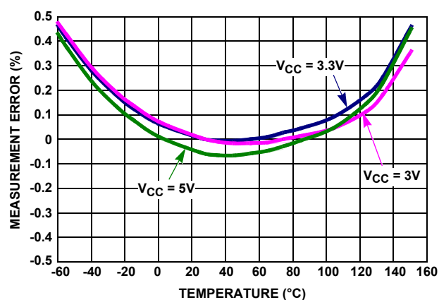
FIGURE 16. PRIMARY V_{SHUNT} MEASUREMENT ERROR vs TEMPERATURE
