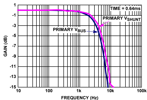
FIGURE 18. PRIMARY V_{SHUNT} AND V_{BUS} vs FREQUENCY
