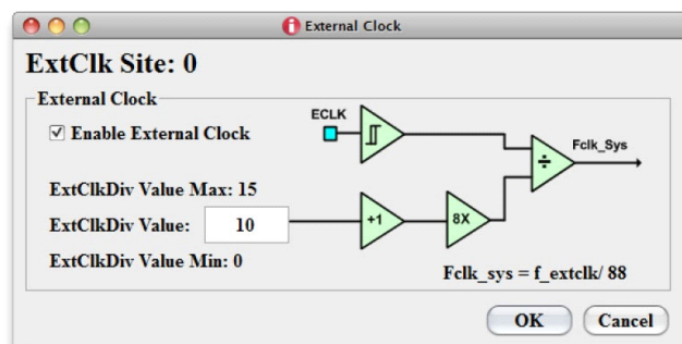
FIGURE 113. EXTERNAL CLOCK MODE
