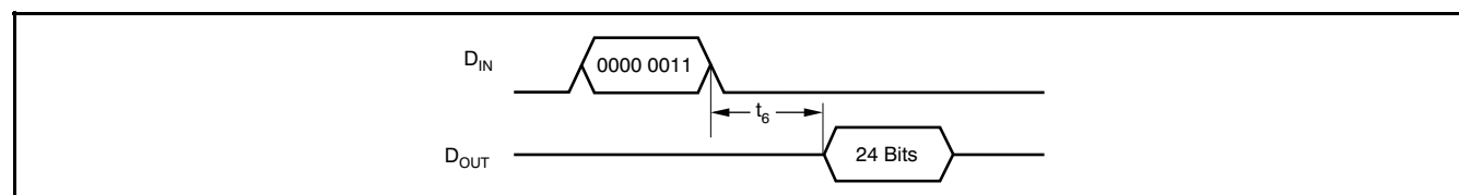
Figure 38. Checksum Command Sequence
