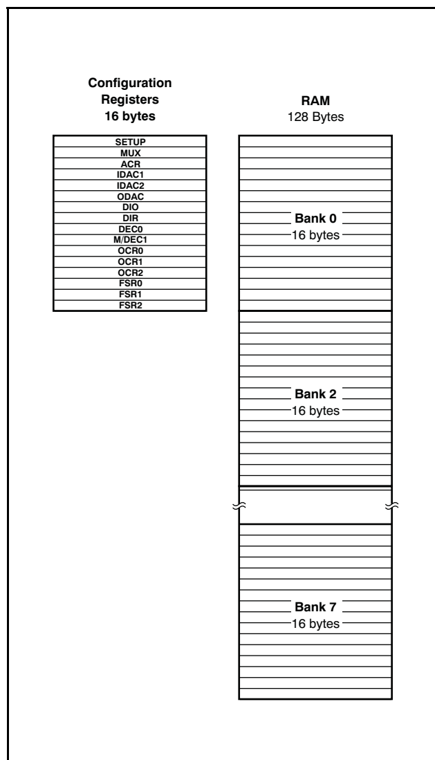
Figure 29. Memory Organization
