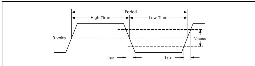
Figure 33-14.Clock Period and Slew Rate Diagram - Differential Measurement
