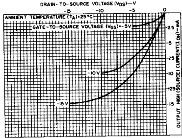
Fig. 6—Typical output high (source) current characteristics.
