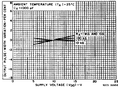
Fig. 21—Typical output pulse-width variations vs. supply voltage.
