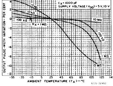
Fig. 24—Typical output pulse-width variations vs. ambient temperature.
