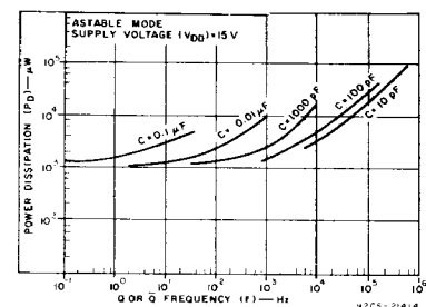
Fig. 28—Typical power dissipation vs. output frequency ( V_{DD} = 15 V).
