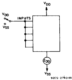
Fig. 29—Quiescent device current test circuit.
