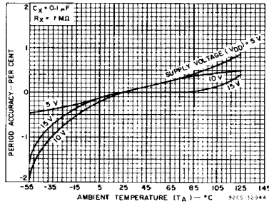
Fig. 15—Typical astable oscillator or Q, \bar{Q} period accuracy vs. ambient temperature (low frequency).
