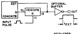
Fig. 35—Implementation of external counter option.
