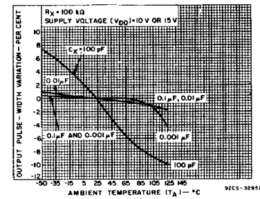
Fig. 23—Typical output pulse-width variations vs. ambient temperature.
