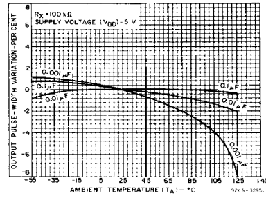
Fig. 22—Typical output pulse-width variations vs. ambient temperature.
