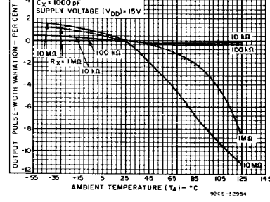
Fig. 25—Typical output pulse-width variations vs. ambient temperature.
