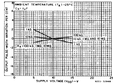
Fig. 19—Typical output pulse-width variations vs. supply voltage.
