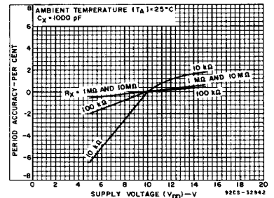
Fig. 13—Typical astable oscillator or Q, \bar{Q} period accuracy vs. supply voltage.
