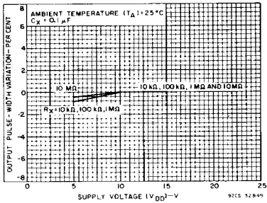
Fig. 20—Typical output pulse-width variations vs. supply voltage.
