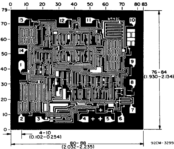
Dimensions in parentheses are in millimeters and are derived from the basic inch dimensions as indicated. Grid graduations are in mils ( 10^{-3} inch).
