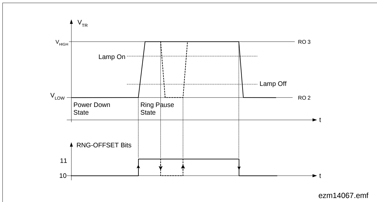
Figure 37 Timing Diagram
