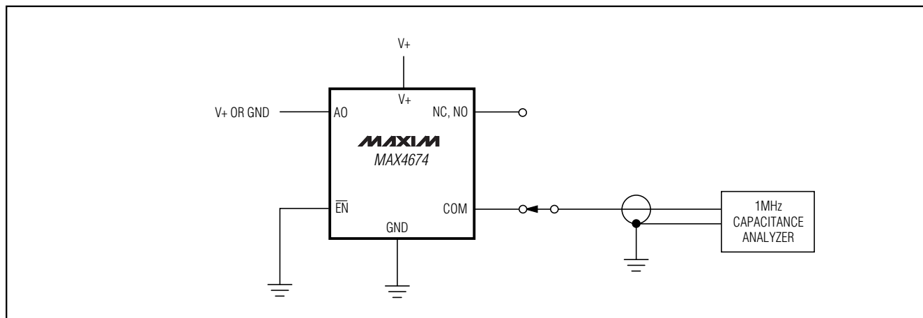
Figure 6. Capacitance
