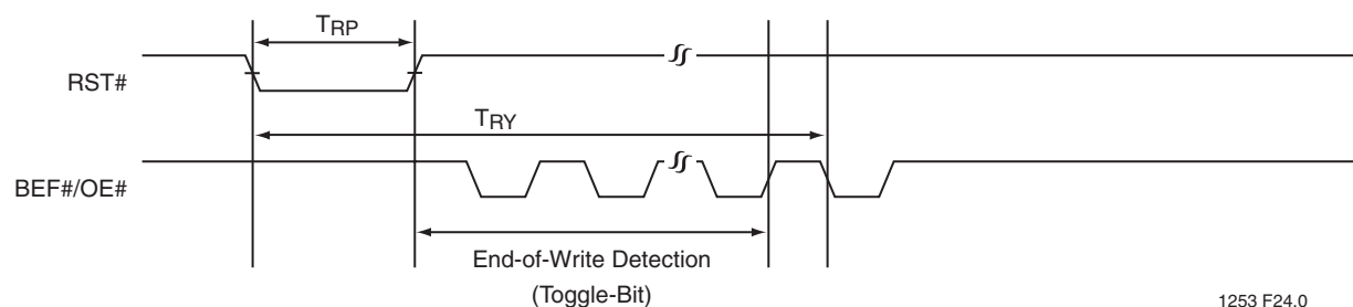
FIGURE 19: RST# TIMING DIAGRAM (DURING PROGRAM OR ERASE OPERATION)
