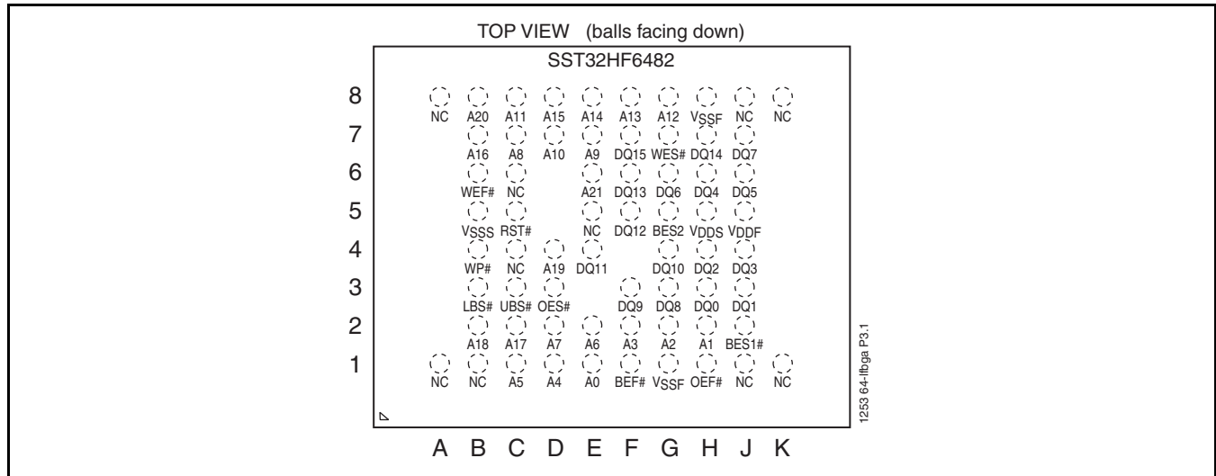
FIGURE 3: PIN ASSIGNMENTS FOR 64-BALL LFBGA (8MM X 10MM)
