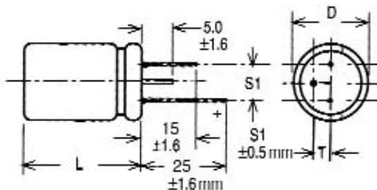
Type 300/300R Three Leads
