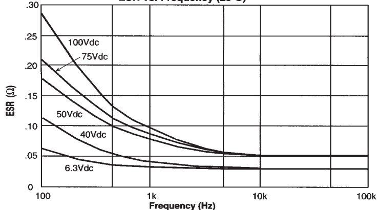
Type 301/301R ESR vs Frequency ESR vs. Frequency ( 25^{\circ}\text{C} )
