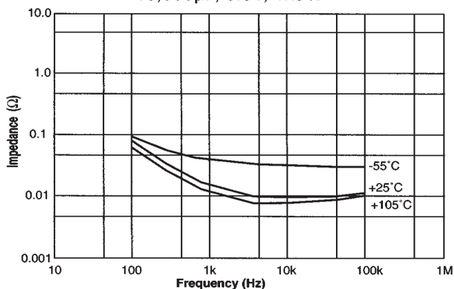
Type 301/301R Impedance vs Frequency 18,000 \mu\text{F} , 6.3V, 1 \times 3\frac{5}{8} "
