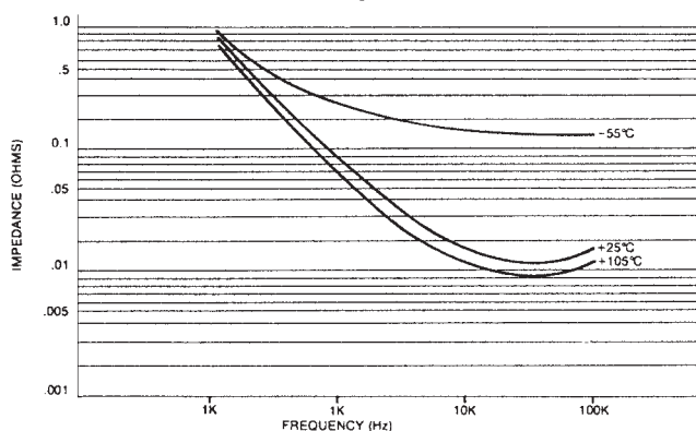
1500 \mu\text{F} 75V, 1'' \times 3\frac{5}{8}'' Impedance-Frequency Characteristics
