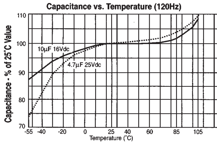
Type 301/301R Capacitance vs Temperature
