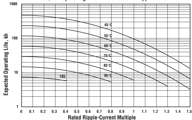
300/301 Operating Life in Kilohours vs Ripple Current
