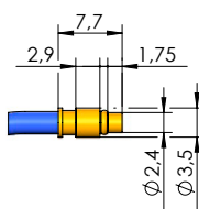
MMPX™-m (straight)
