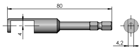
BIT-HFS-810 M
