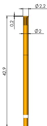
KS-215 M1,6-F-R
