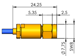
PC3.5-m (straight)
