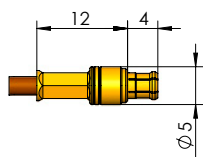
MCX-plug (straight)*
