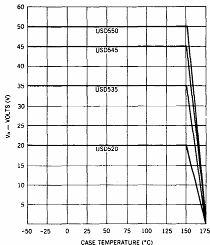
V_{R(MAX)} Rating vs Case Temperature
