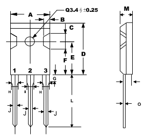
TO-247 (3P)
