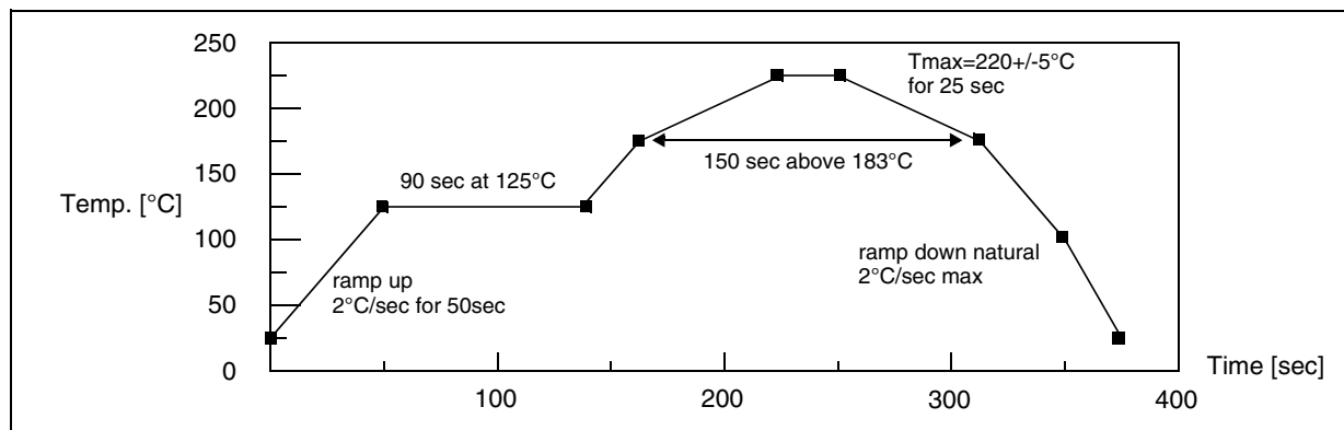
Figure 92. Recommended Reflow Soldering Oven Profile (MID JEDEC)
