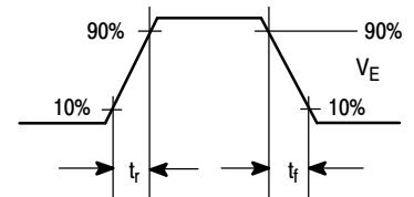
Figure 14. Emitter-Follower Configuration and Waveform
