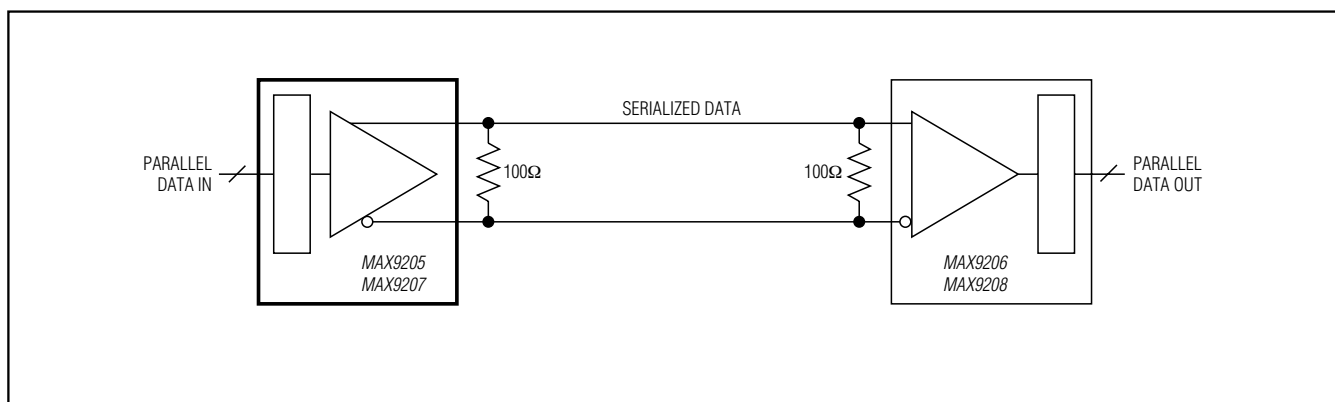
Figure 11. Double-Terminated Point-to-Point
