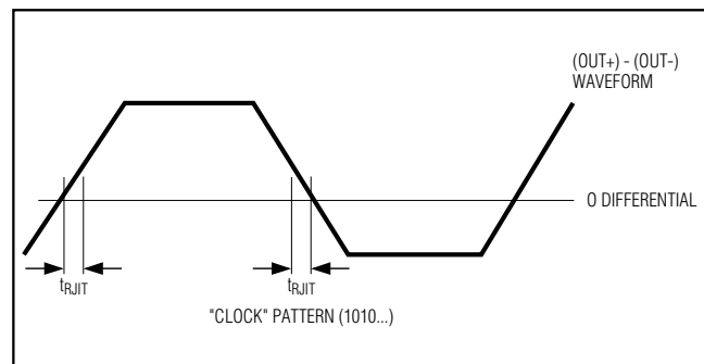
Figure 10. Definition of Random Jitter ( t_{RJIT} )
