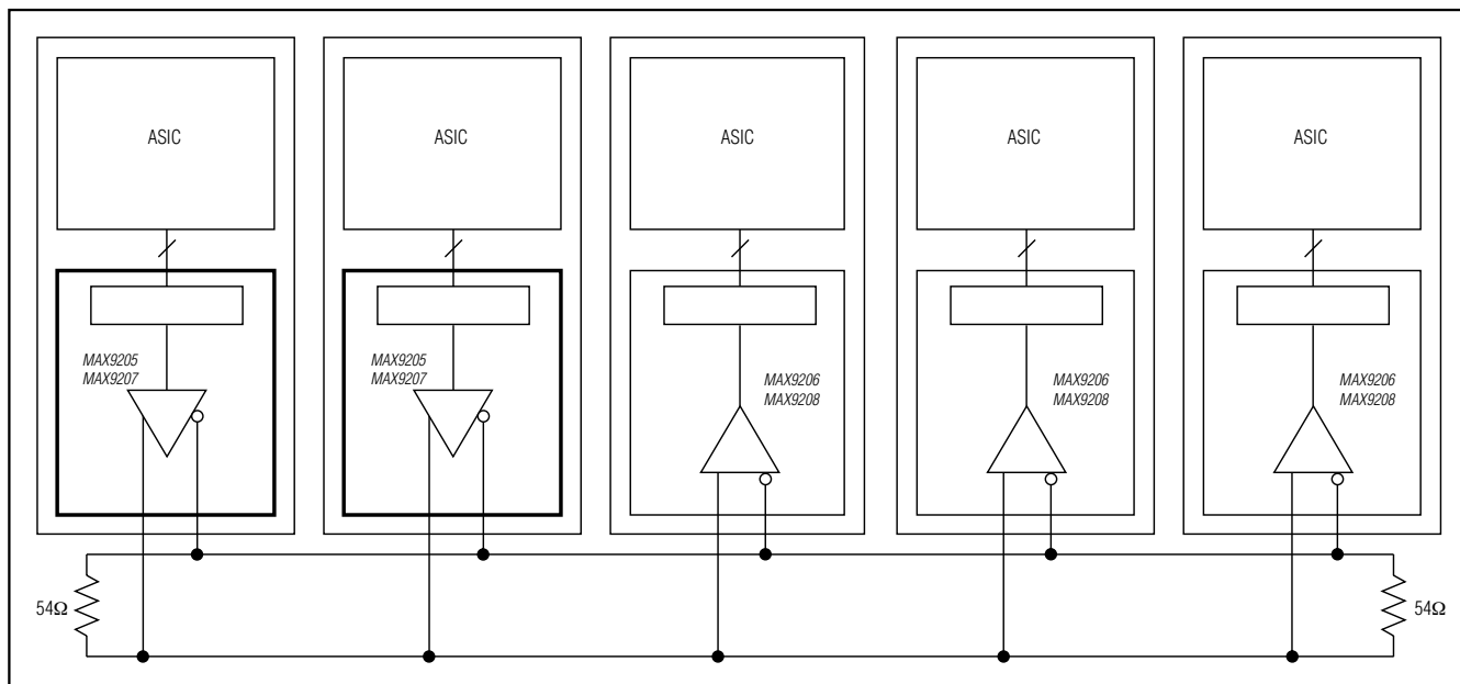
Figure 14. Multipoint
