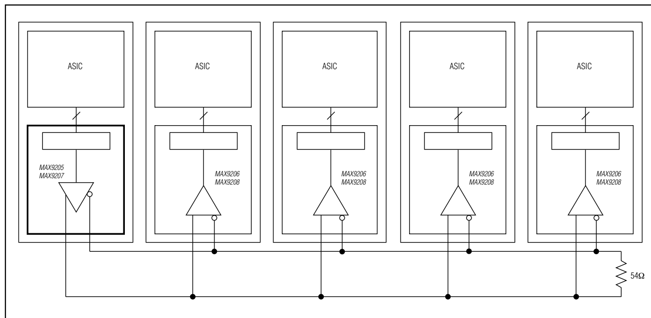
Figure 12. Multidrop
