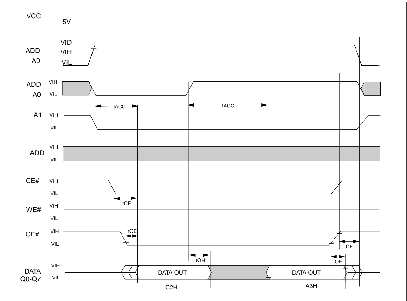
Figure 21. SILICON ID READ TIMING WAVEFORM
