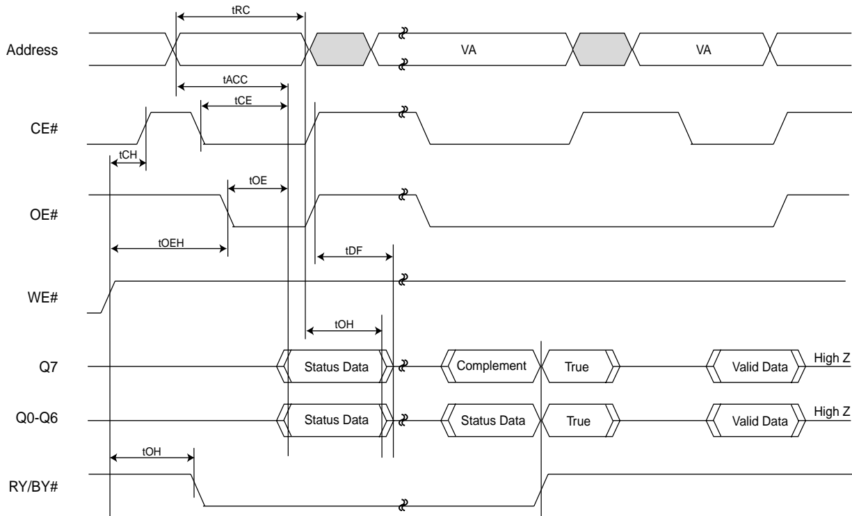
Figure 22. DATA# POLLING TIMING WAVEFORMS (DURING AUTOMATIC ALGORITHMS)
