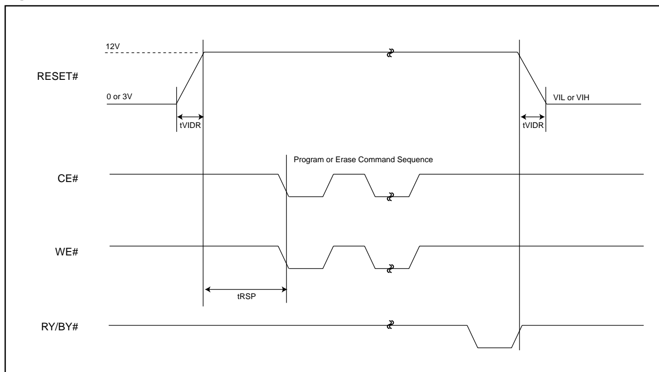
Figure 19. TEMPORARY SECTOR GROUP UNPROTECTED WAVEFORMS
