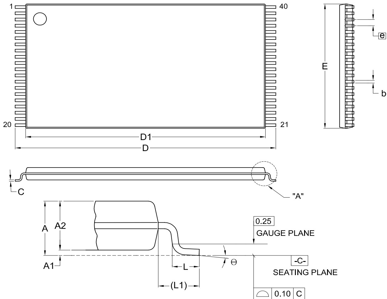
DETAIL "A"
