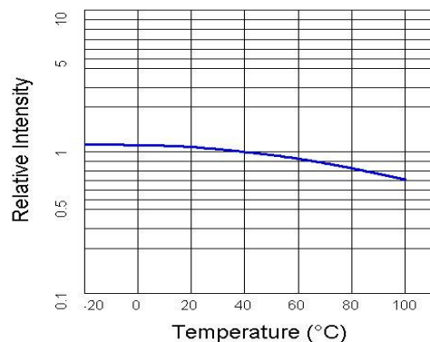
Relative Intensity vs. Ambient Temperature Pulsed 20mA; 300us pulse, 10ms period
