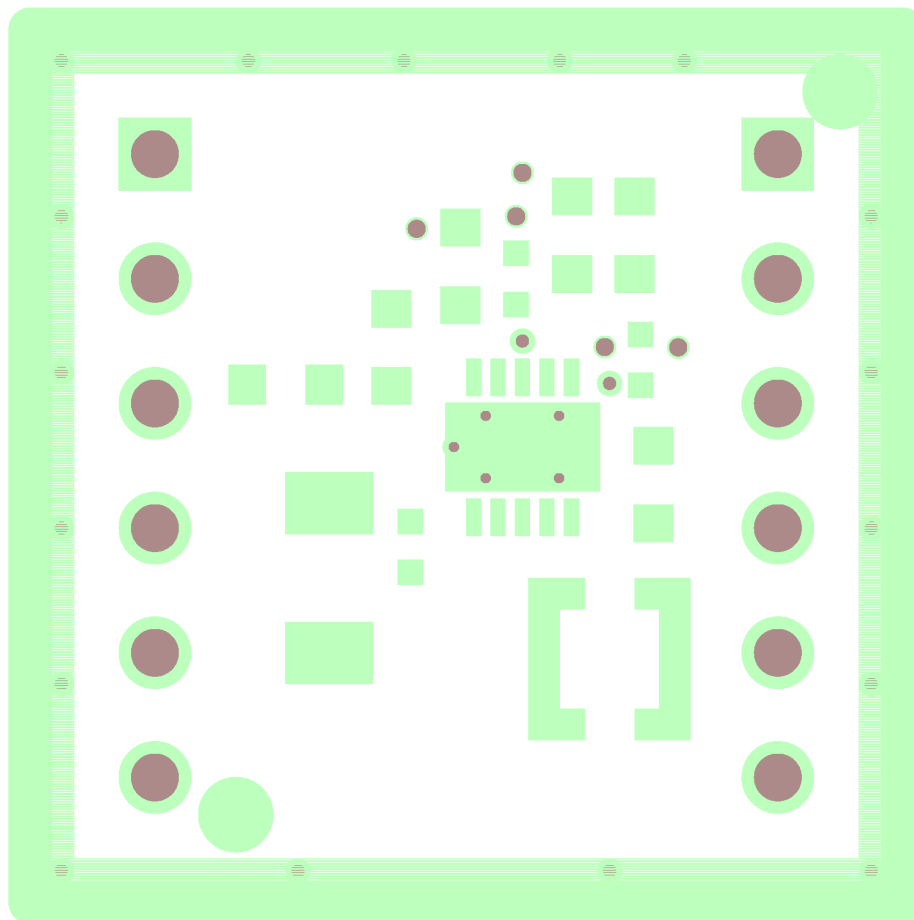
Figure 5. SMP-TPS61201-MVK Board Solder Mask – Top Side
