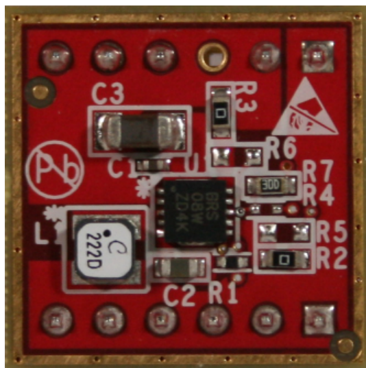
Figure 1. SMP-TPS61201-MVK Submodule
