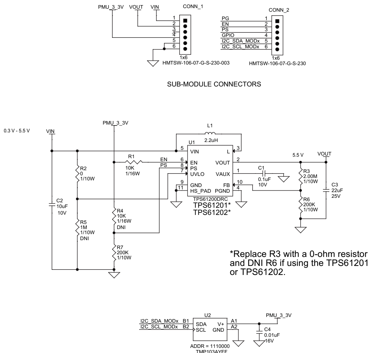
Figure 12. SMP-TPS61201-MVK Schematic
