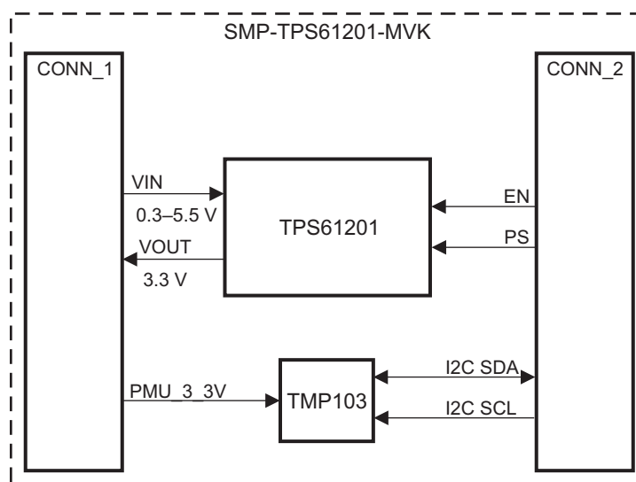
Figure 2. SMP-TPS61201-MVK Block Diagram
