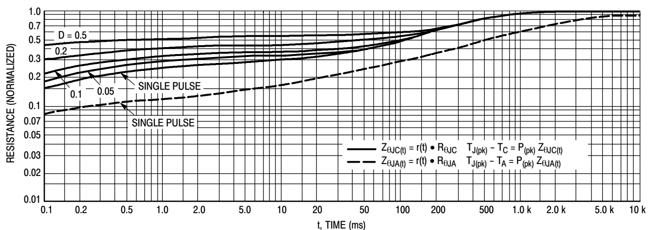
Figure 17. Thermal Response
