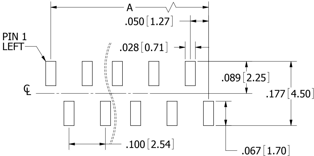
RECOMMENDED PCB SMD LAYOUT GRP B _ 1 VWTC-RC
