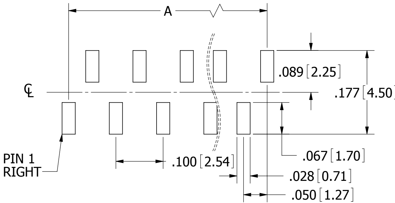
RECOMMENDED PCB SMD LAYOUT GRP B _ 1 VWTD-RC
