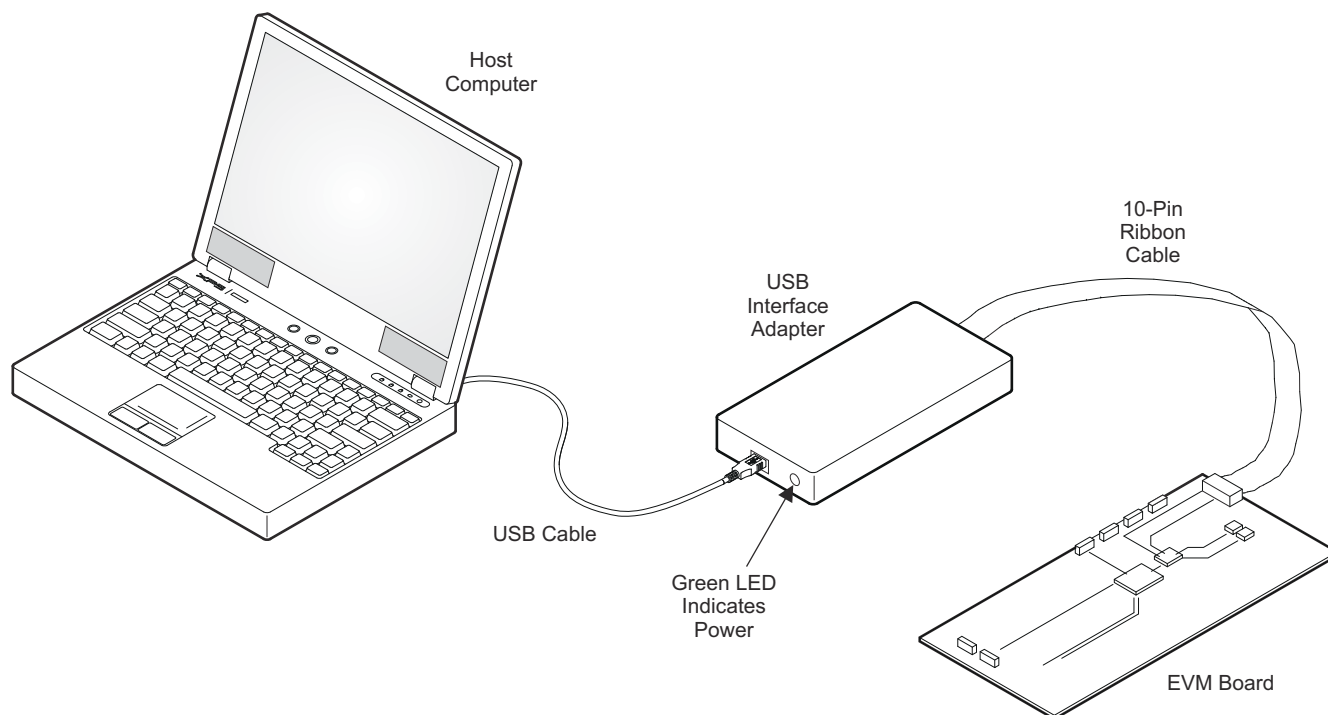
Figure 5-2. USB Interface Adapter Quick Connection Diagram
