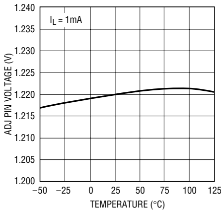
LT1762 ADJ Pin Voltage
