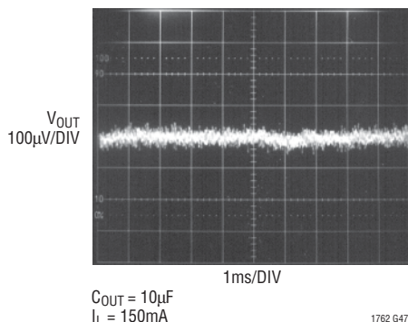
LT1762-5 10Hz to 100kHz Output Noise C_{BYP} = 0.01\mu F
