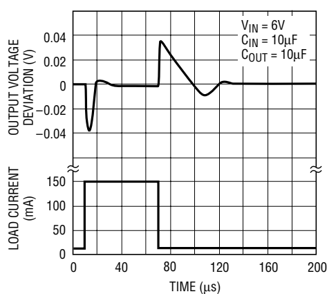
LT1762-5 Transient Response C_{BYP} = 0.01\mu F
