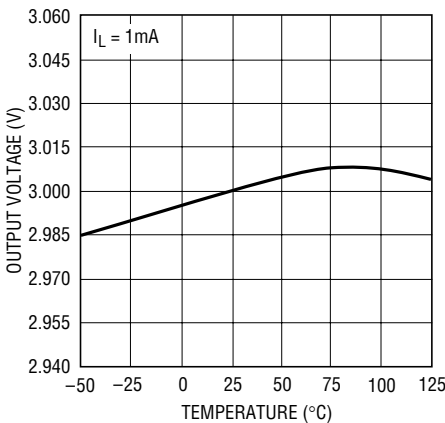
LT1762-3 Output Voltage
