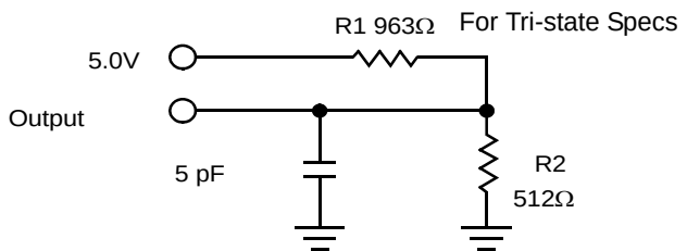
Figure 6. AC Test Loads
