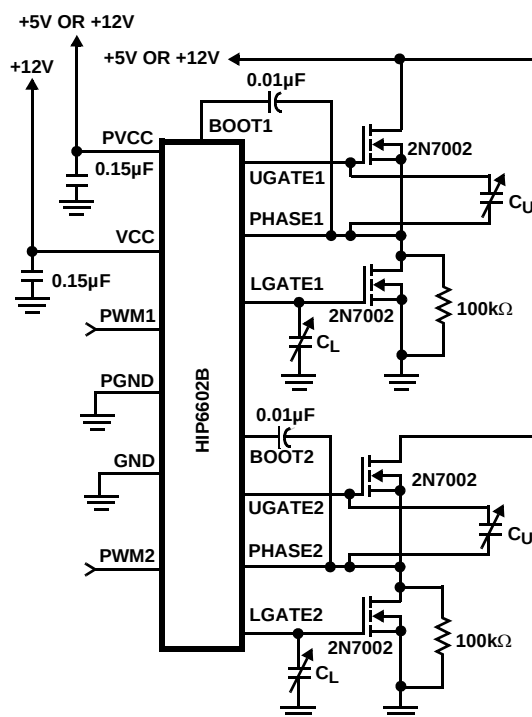
FIGURE 1. HIP6602B TEST CIRCUIT
