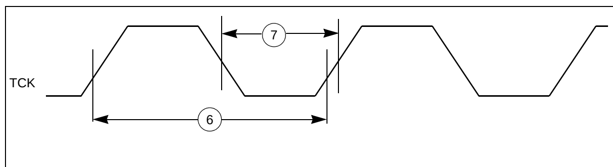
Figure 19. Nexus event trigger and test clock timings
