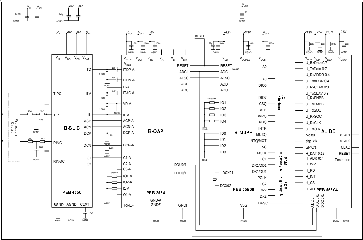
Figure 5-1 Application Circuit
