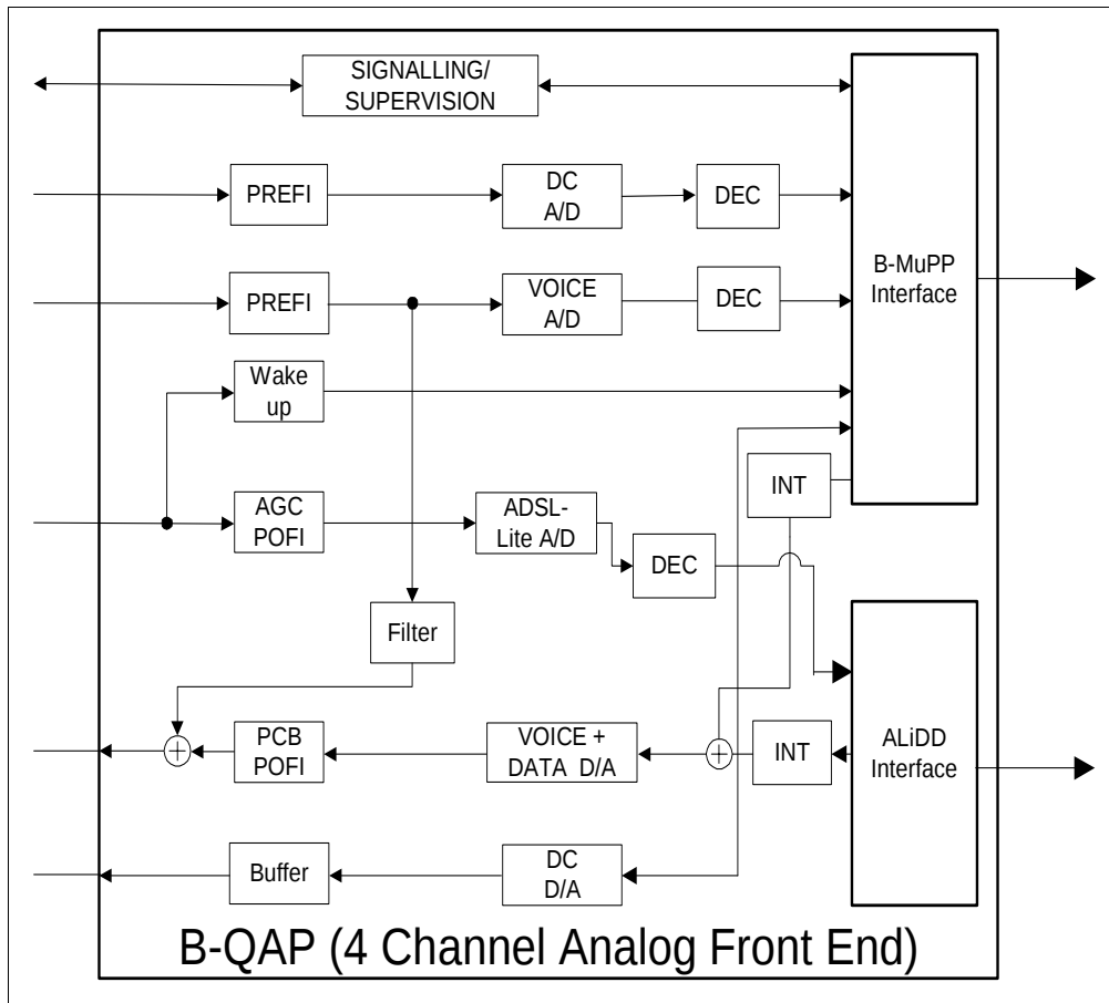
Figure 2-2 ADSL-Lite Analog Frontend B-QAP (Only 1 of 4 Channels Shown)
