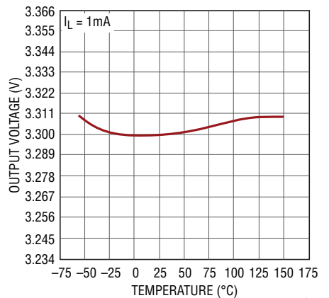
LT3060-3.3 Output Voltage
