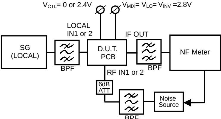
Noise Figure Measuring Block Diagram
